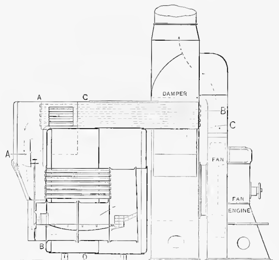
FIG. 3.—VERTICAL LONGITUDINAL SECTION.
